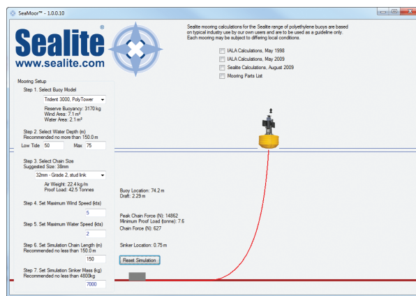
Mooring solutions are calculated using Sealite's advanced mooring calculator
